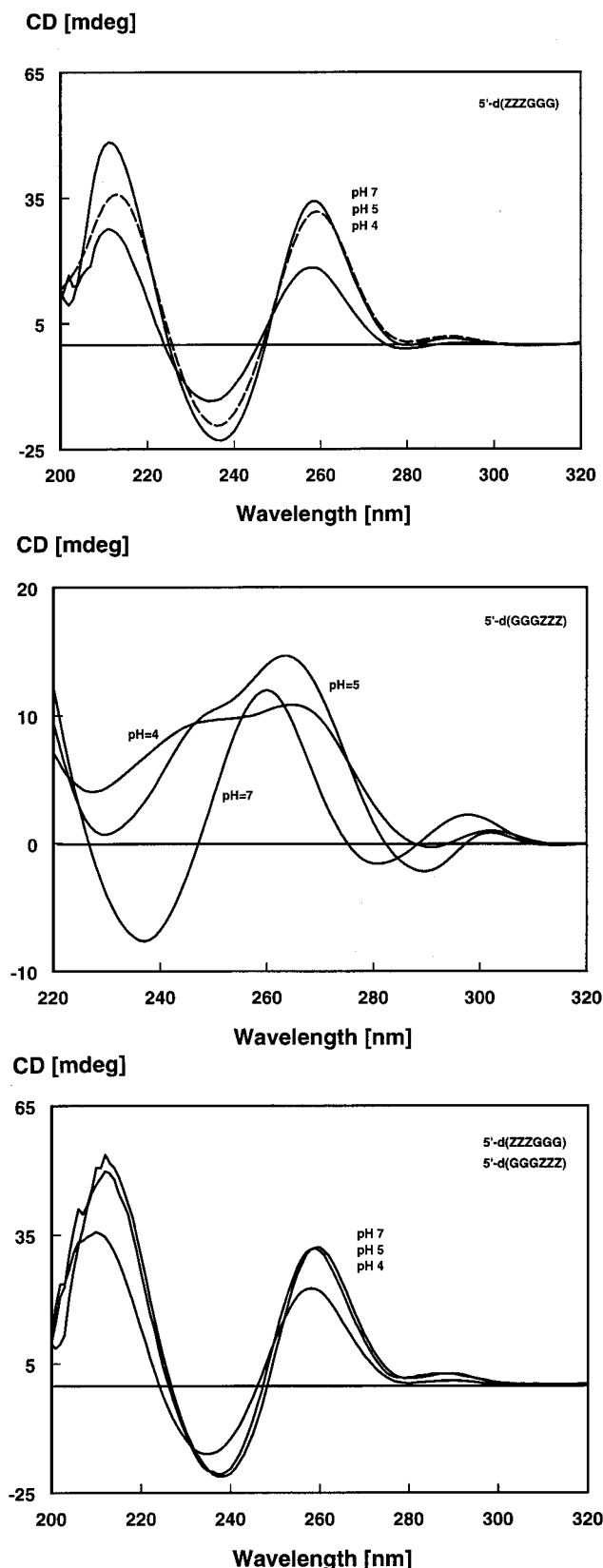
Figure 1. pH-dependent CD spectra a) of self-complementary oligomer d(ZZZGGG) ( 33 ), b) of self-complementary oligomer d(GGGZZZ) ( 34 ) and c) of duplex d(ZZZGGG)–d(GGGZZZ) ( 33 · 34 ), measured at 0 °C in 60 mM sodium cacodylate, 1 M NaCl, and 100 mM MgCl 2 at pH = 4.0, 5.0 and 7.0; the oligomer concentration was 10 μM of single-strands
